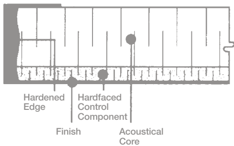
Construction Cross Section
